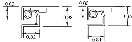
Cross Section of 14 gauge Body & Door Cross Section of 16 gauge Body & Door
